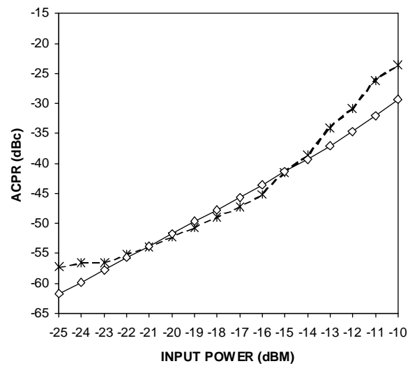
Figure 3: Measured and calculated ACPR, *-measured, dimonds-calculated.
